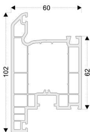
PRO10 Outward Door Profile
