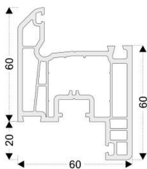
PRO02 Sash Profile
