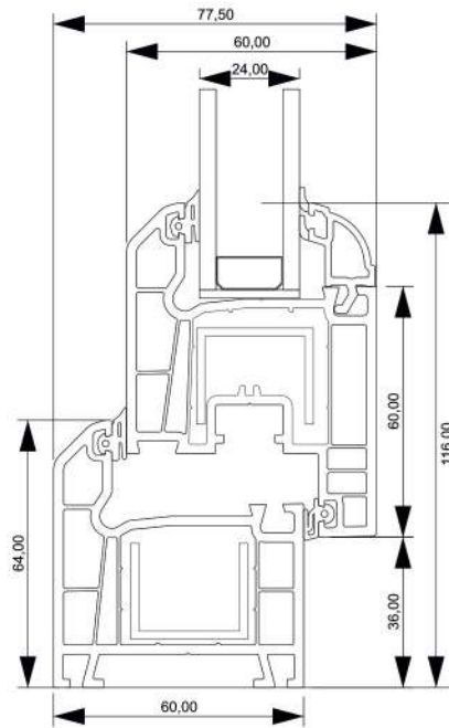
Frame - Sash Connection Section
