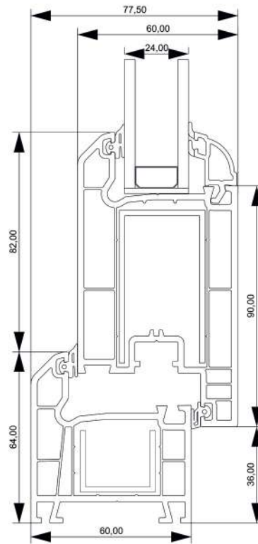
Frame - Inward Opening Door Sash Connection Section
