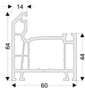
PRO01 Frame Profile
