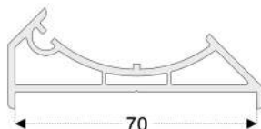
PRO331 Corner Profile - 60mm
