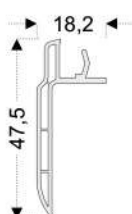
PRO38 Nailed Trim Profile (60mm Series)
