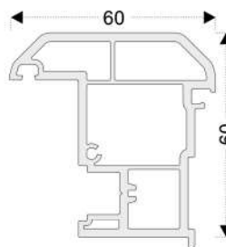
PRO12 French Casement Mullion Prf.
