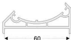
PRO33 Corner Profile - 60mm
