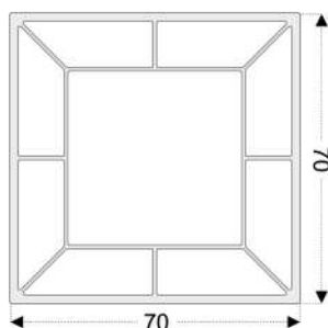
PRO80 Box Profile - 70x70mm (70mm Series)
