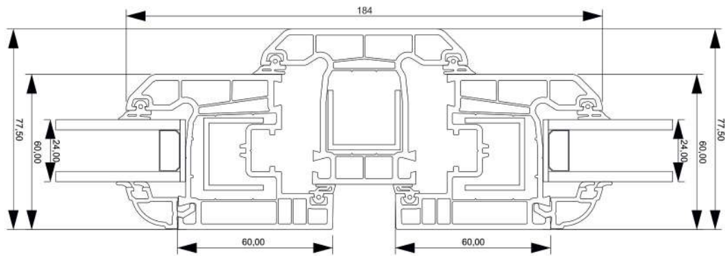
Sash - Mullion - Sash Connection Section
