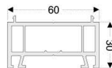
PRO14 Rising Profile - 30mm (60mm Series)
