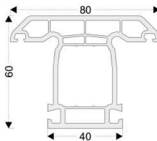
PRO03 Mullion Profile
