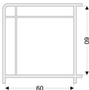
PRO36 Box Profile - 60x60mm (60mm Series)
