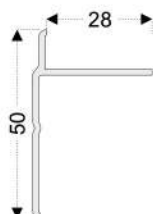
PRO35 T Trim Profile (60mm Series)
